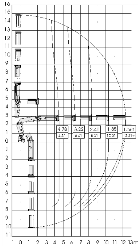
240.2-12.5/4 (A4)
