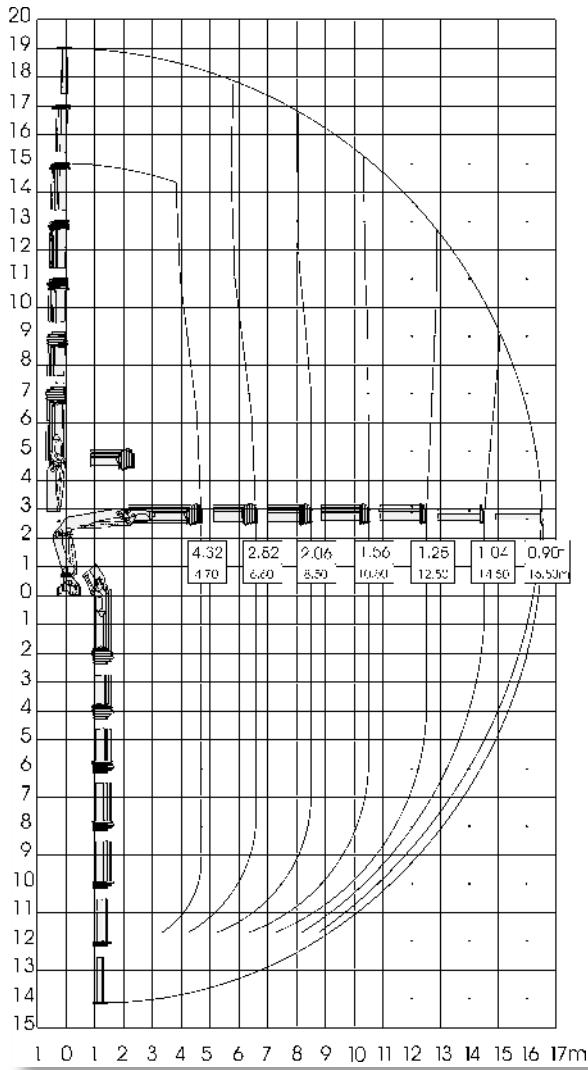
240.2-16.7/6 (A6)
