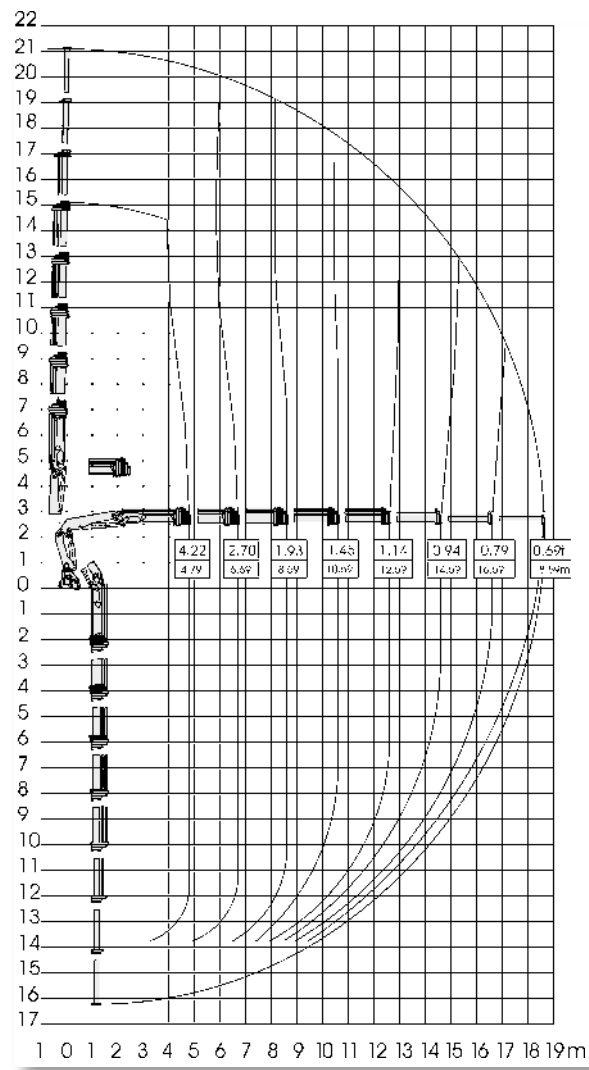
240.2-18,8/7 (A7)
