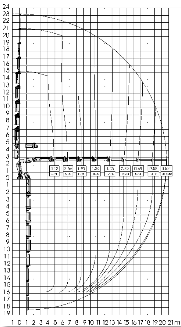
240.2-20,7/8 (A8)
