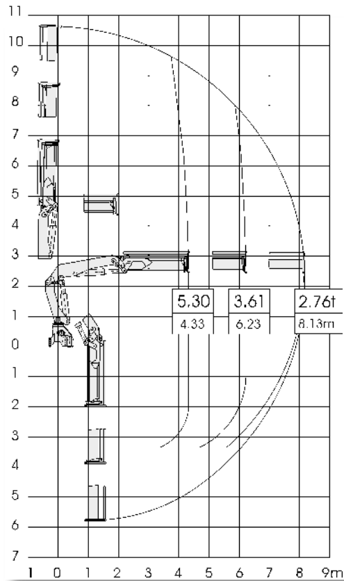
240.2-12.5/4 (A4)
