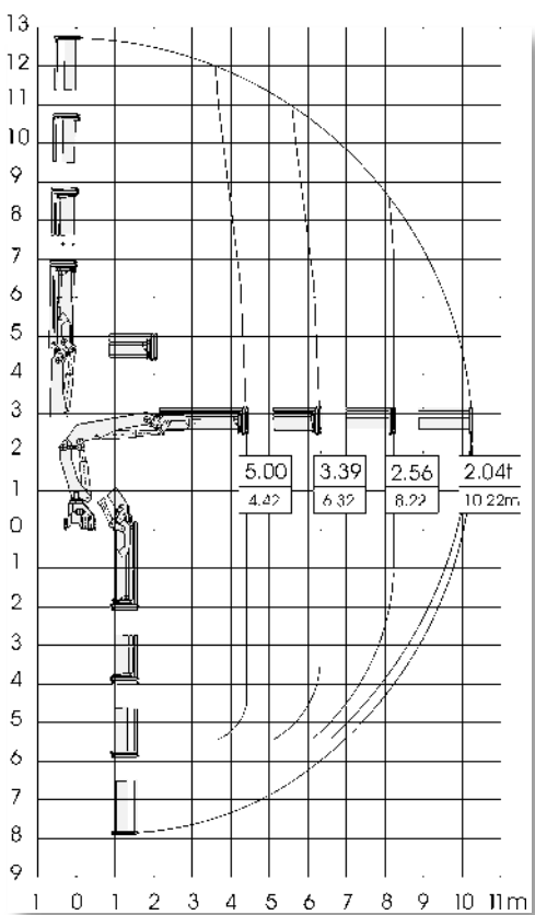
240.2-10.4/3 (A3)
